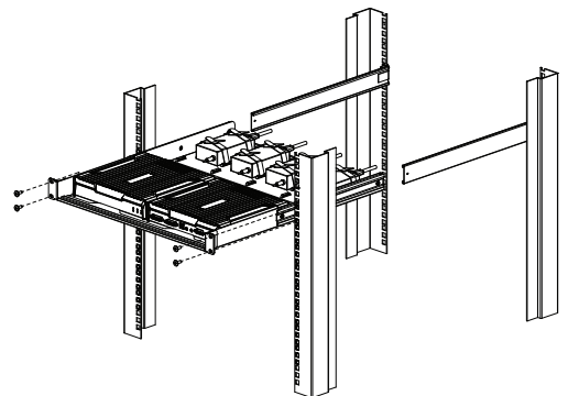
KE6948A 2-in-1U KE6948A Rack Mount Kit (2K-0013)
